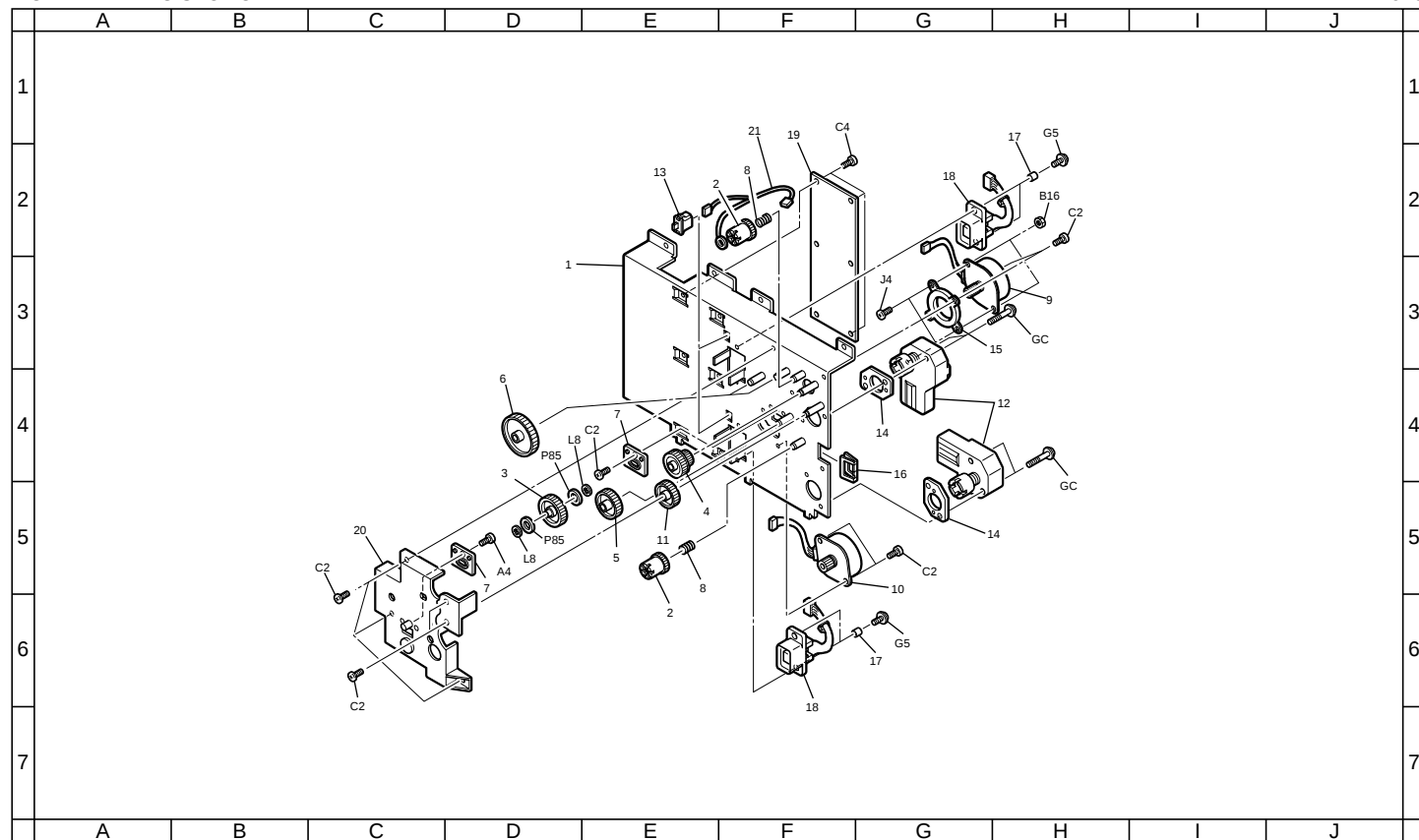
FIG. 2 DRIVING SECTION
